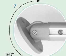
Sloped walls, acute angles: the Vario wall connector RVS/WAV compensates for and levels out asymmetries up to 180° and length differences up to +/- 5 mm.
