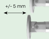
Sloped walls, acute angles: the Vario wall connector RVS/WAV compensates for and levels out asymmetries up to 180° and length differences up to +/- 5 mm.
